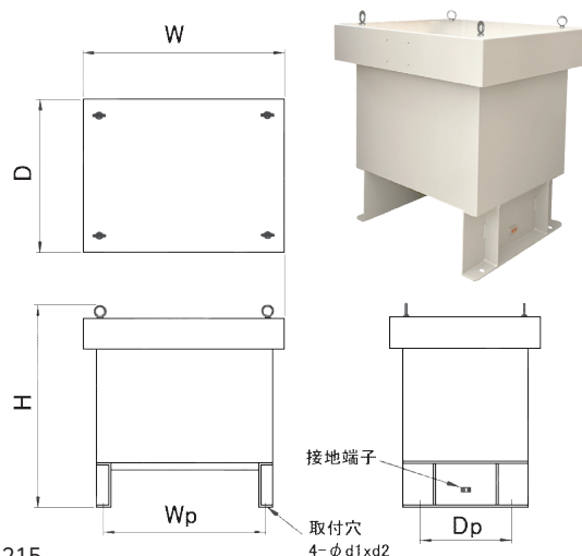
図-B2
