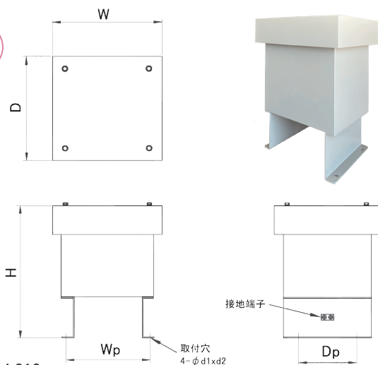
図-B1
